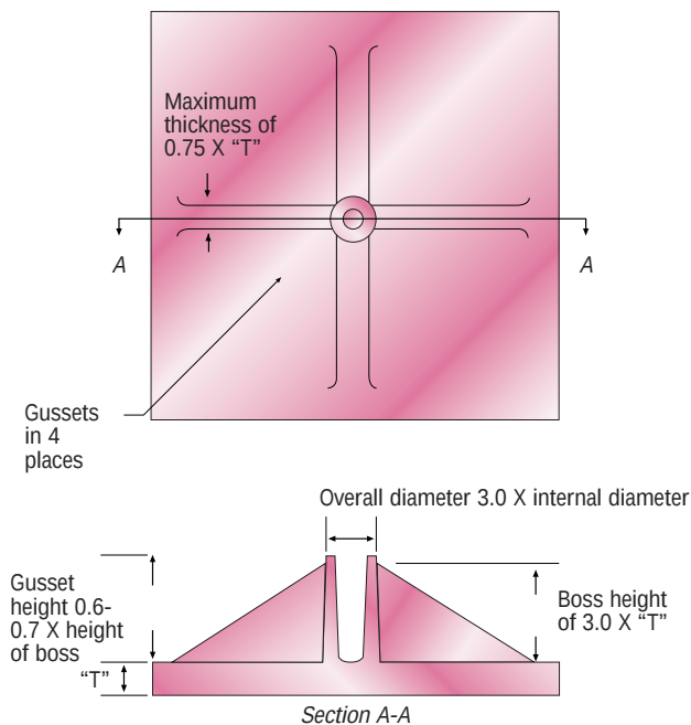
Free Standing Boss With Four Gussets
